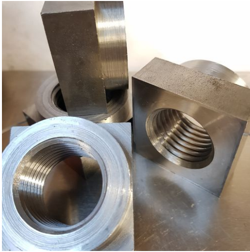
Large Square Nuts with Spigot
