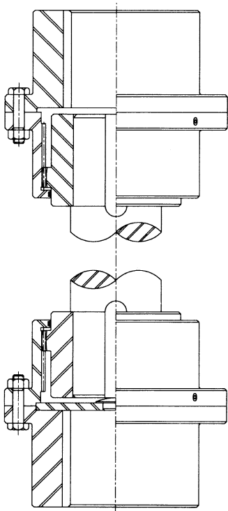
FIG. C TANDEM - VERTICAL
