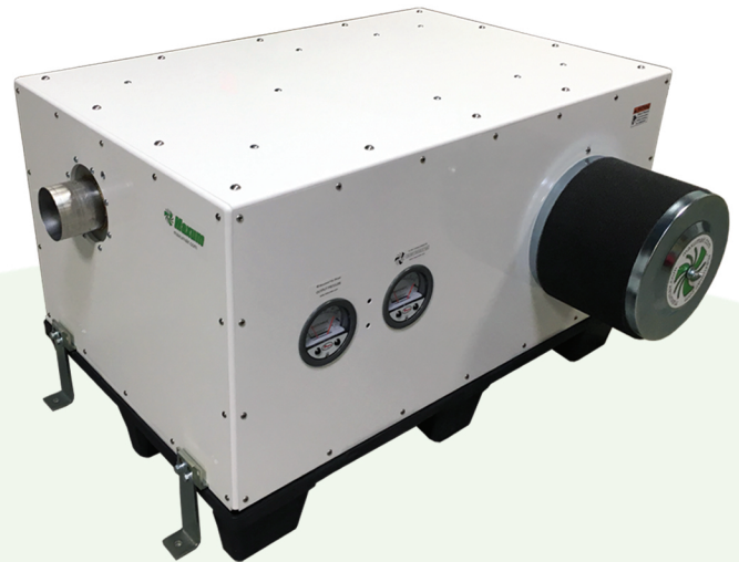
Horizontal "S" Enclosure - Side-mounted gages and filter
