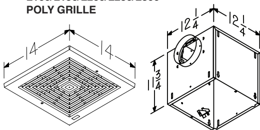
L100/L150/L200/L250/L300 POLY GRILLE
