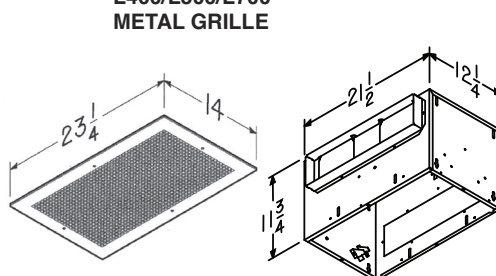
L400/L500/L700 METAL GRILLE
