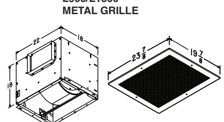
L900/L1500 METAL GRILLE
