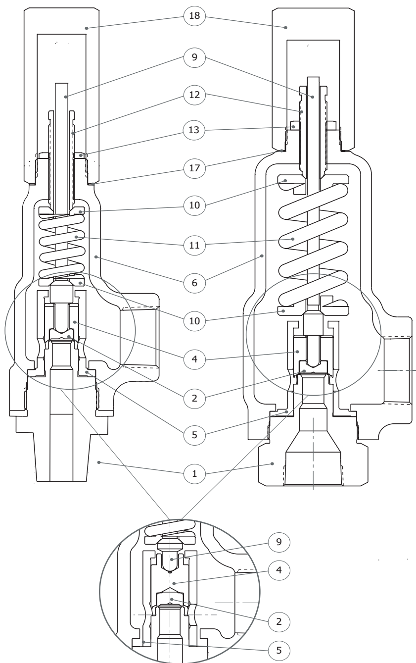
DVSC-33 Metal Seat Valve Construction Model : L & M
