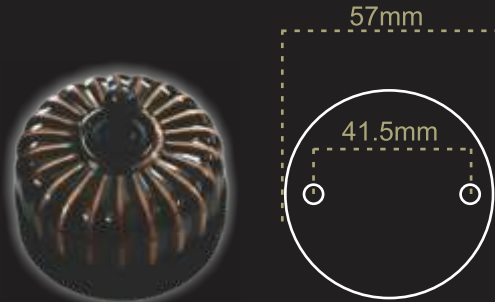
MOUNTING DIMENSION OF ALL MODULES
