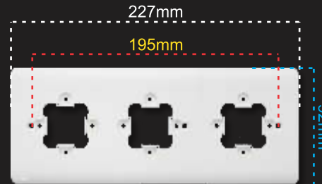
COVER FRAME FOR 3 MODULE SUITABLE FOR 8"X3" FRAME
