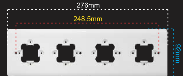
COVER FRAME FOR 4 MODULE SUITABLE FOR 10"X3" FRAME
