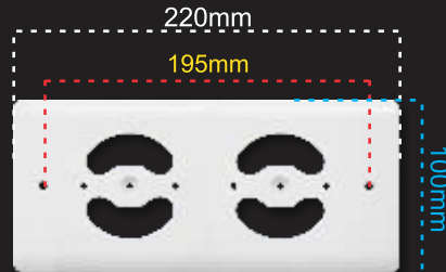
COVER FRAME 2 MODULE FOR POWER SWITCH & OUTLET SUITABLE FOR 8"X3" FRAME
