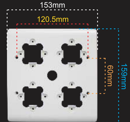
COVER FRAME FOR 4 MODULE SUITABLE FOR 5"X5" FRAME
