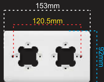
COVER FRAME FOR 2 MODULE SUITABLE FOR 5"X3" FRAME
