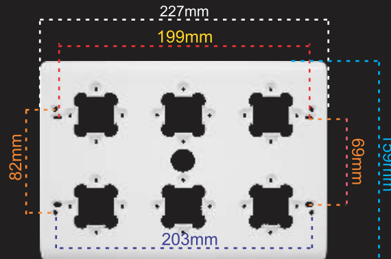
COVER FRAME FOR 6 MODULE SUITABLE FOR 8"X6" FRAME
