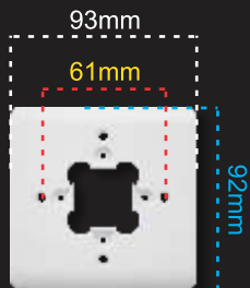
COVER FRAME FOR 1 MODULE SUITABLE FOR 3"X3" FRAME
