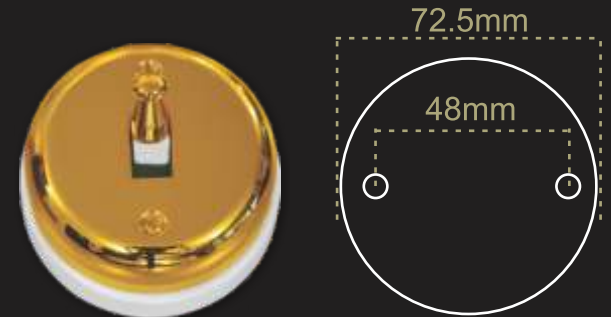
MOUNTING DIMENSION OF LARGE MODULES
