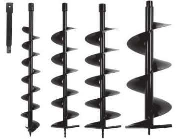
53.Auger Bits 6" / 8" / 10" / 12"
