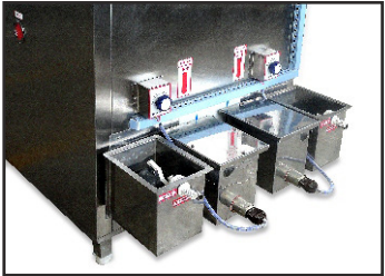
Stand by Steam Generator system
