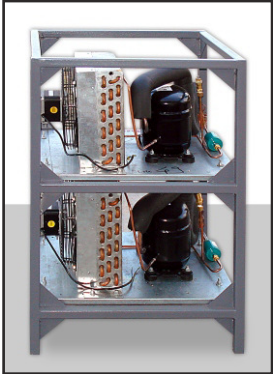
Stand by Refrigeration system
