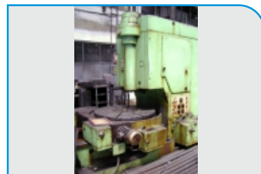
Russian Gear Shaper 5B161 1250mm x 12 module
