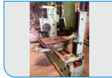
TOS H63 Table Type X-900 Y-700 With Facing Chuck and Tailstock
