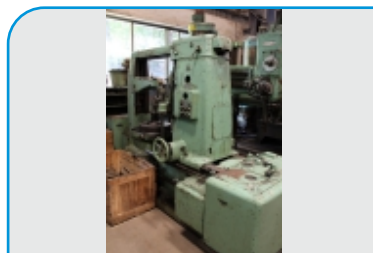
TOS FO 6 Gear Hobbing 600 x 6 module with Tangential attachment and change gears
