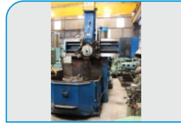
TOS SKJ8F VTL 800mm Chuck, 1050mm Swing, 650mm Height Hardened Bed with Ball Screws
