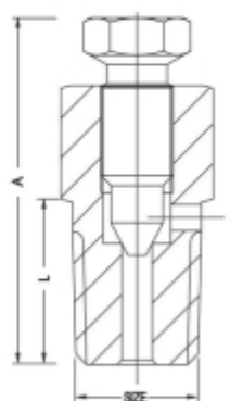
DRAIN VALVE
