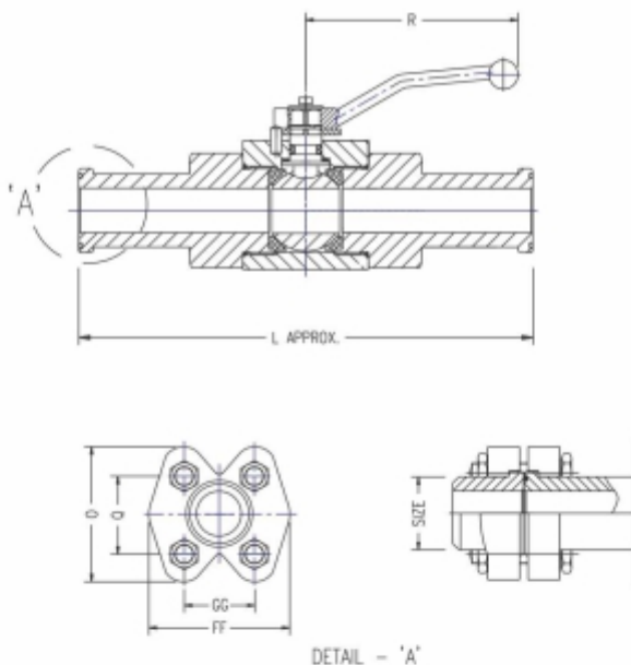
ASSEMBLY SAE FLANGE WITH BUTT WELD SLEEVE.
